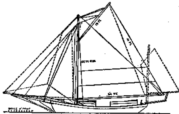
Sail-plan of the SPRAY
