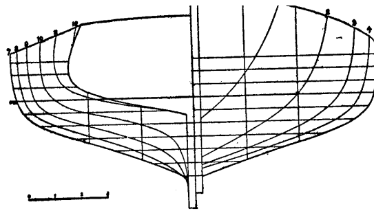
Body-plan of the Spray .
